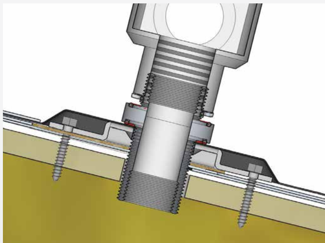
Side View of Assembly Installed on Asphalt Shingle
